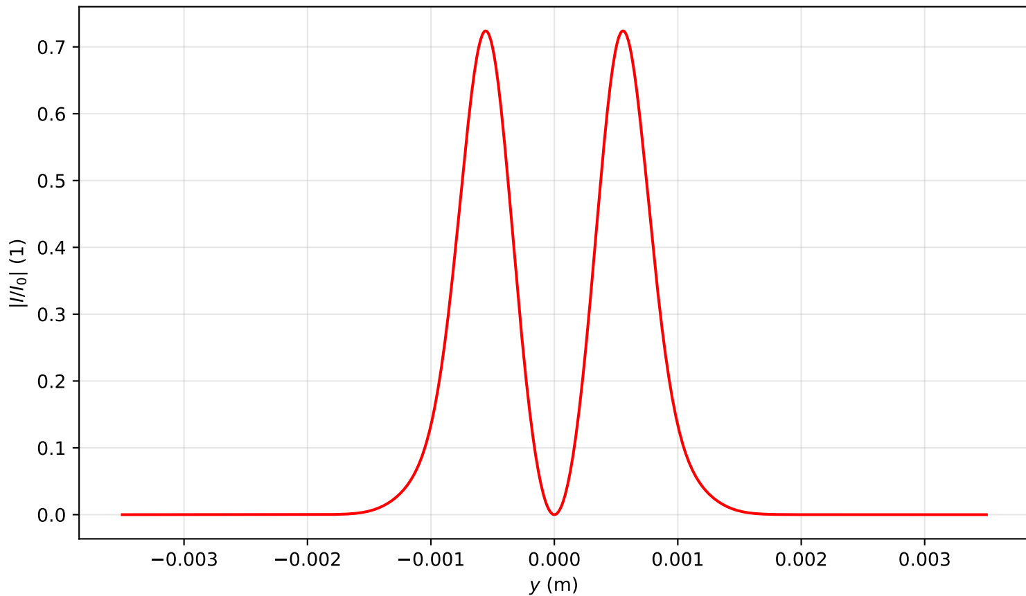
Intensity profile I(x=0, y, z=0.796)/I_0 , P_{in}=2.0P_{cr} , artificial time
